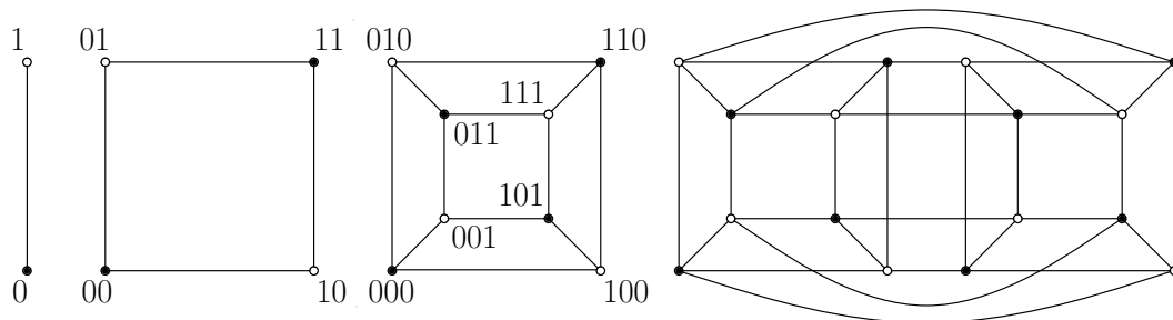
Figure 1.1: Examples of hypercubes Q_n for n = 1, 2, 3, 4 .
