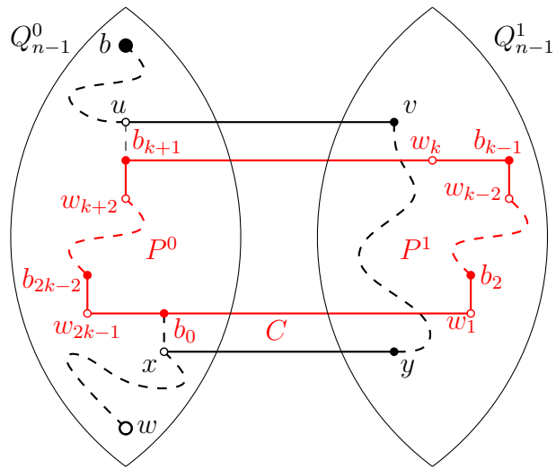
Figure 5.11: Case 1 in the proof of Theorem 24.
