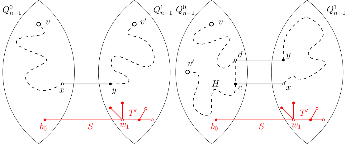
Figure 5.7: Cases 1 and 2 in the proof of Theorem 23 with S as an example of a black-balanced tree on 7 vertices.
